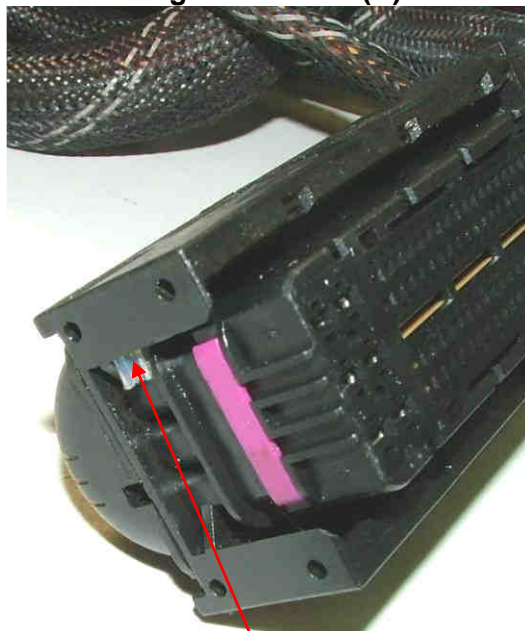
Big connector (B)
